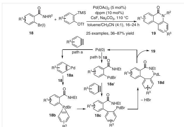
Scheme 9 Phenanthridinones by annulation of o -halobenzamides with arynes
