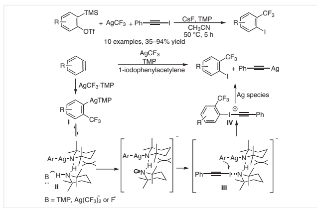
Scheme 35 Ag-mediated trifluoromethylation-iodination of arynes
