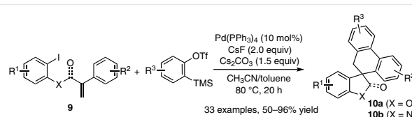
Scheme 6 Pd-catalyzed spirocyclization
