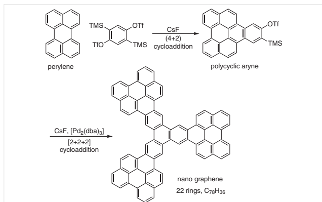
Scheme 31 Synthesis of nanographene from a polycyclic arynes
