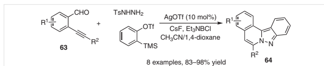
Scheme 38 Pyrazolo[5,1- a ]isoquinolines by three-component coupling of aryne, benzaldehyde, and sulfonylhydrazine
