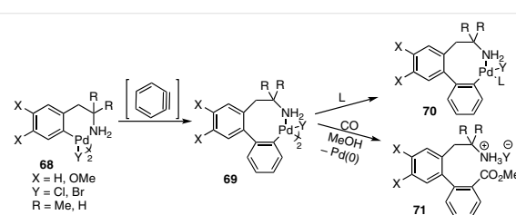
Scheme 44 Synthesis of unnatural amino acids
