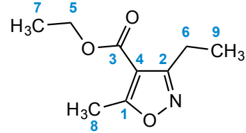
Ethyl 3-Ethyl-5-methyl-4-isoxazolcarboxylate
