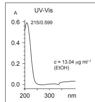
Ethyl 3-Ethyl-5-methyl-4-isoxazolcarboxylate
