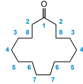
Cyclopentadecanone (Exaltone®)
