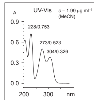
4-Hydroxy-3-methoxybenzaldehyde Vaniline
