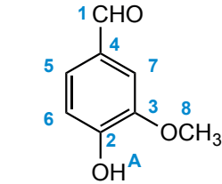
4-Hydroxy-3-methoxybenzaldehyde Vaniline
